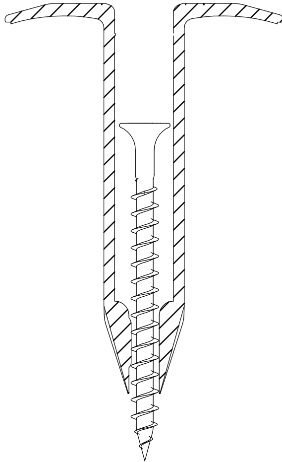
Eurofast EDS-H 5,0 x L
