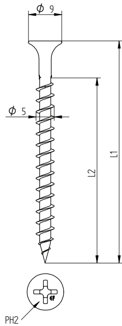
Eurofast EDS-H 5,0 x L
