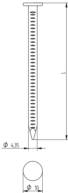
Eurofast ISPC Nail \phi 4,35
