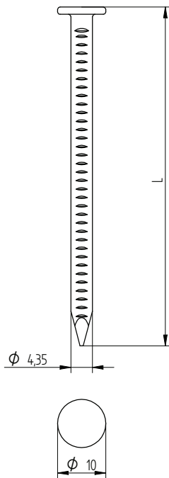
Eurofast ISPC Nail A2 \phi 4,35
