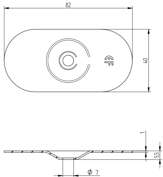
Eurofast DVP-DF-8240R
