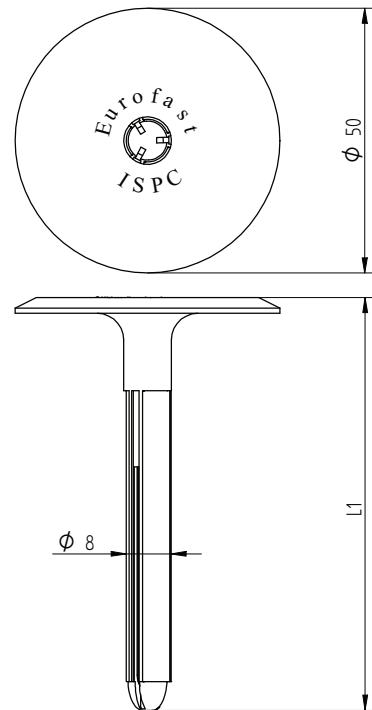
Eurofast ISPC Plug \phi 50
