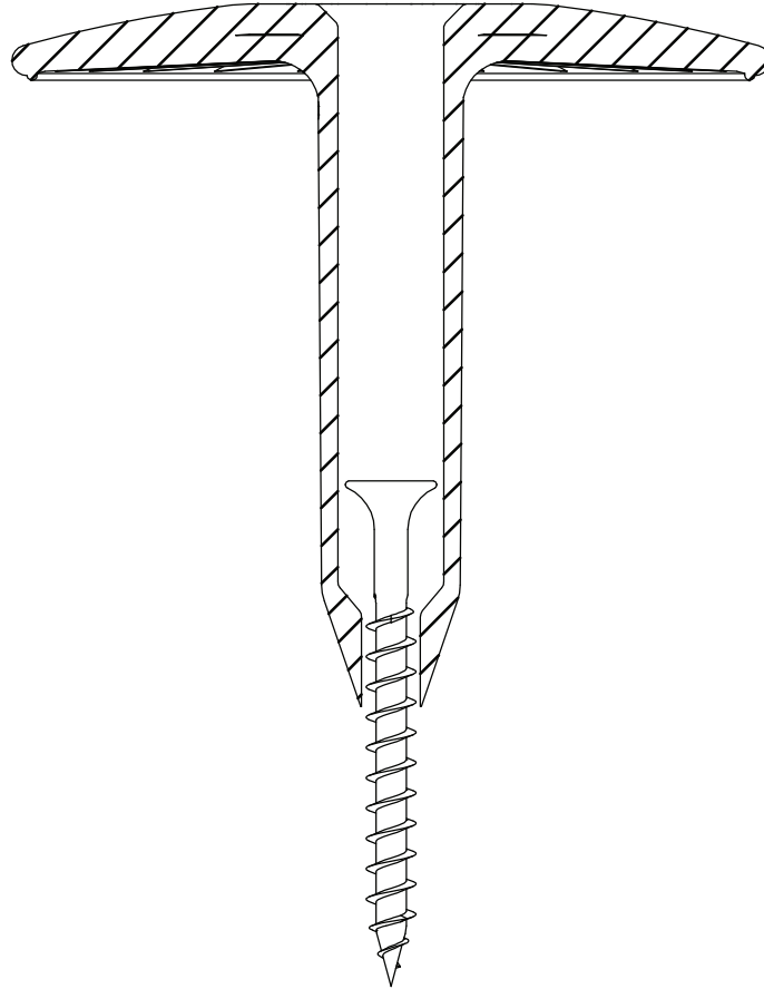
Eurofast EDS-H 5,0 x L
