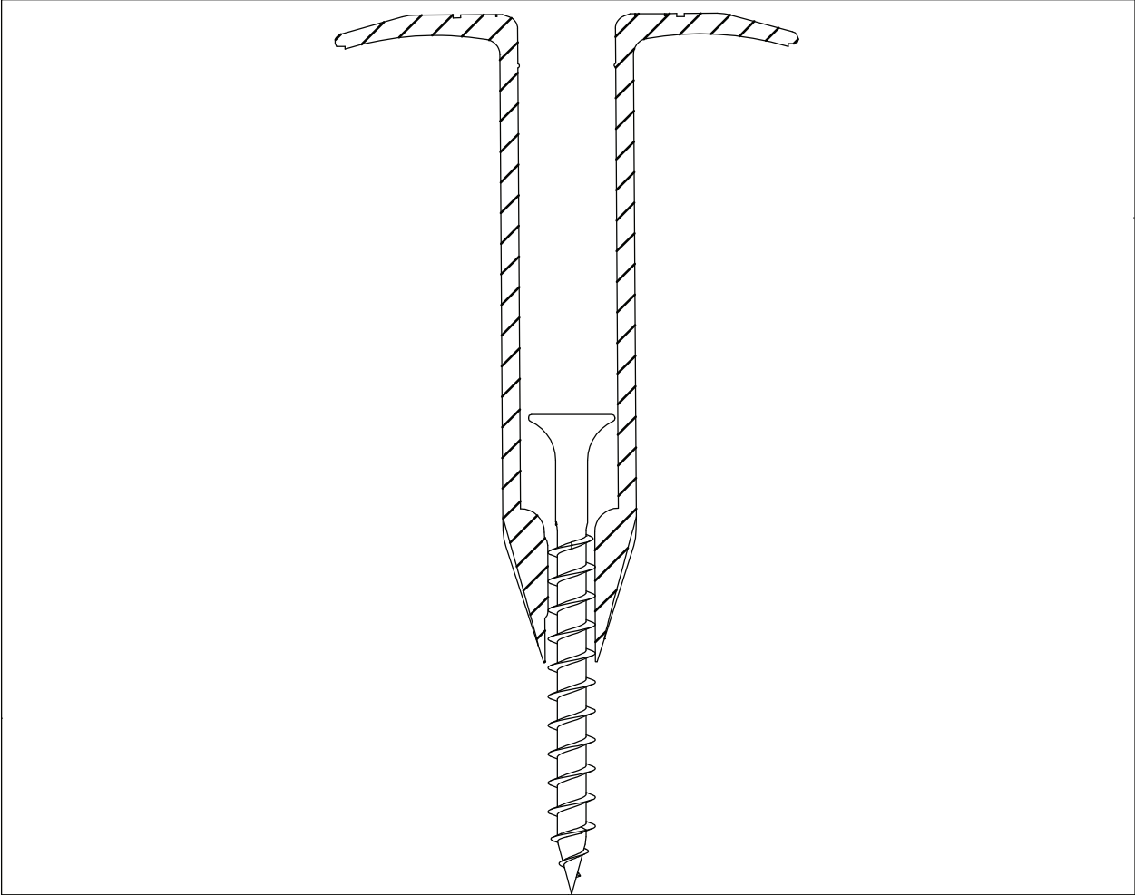
Eurofast EDS-H 5,0 x L
