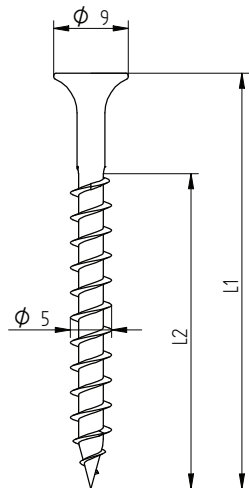
Eurofast EDS-H 5,0 x L
