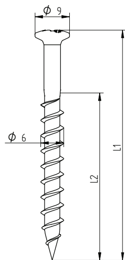
Eurofast GBS-A2 6,0 x L
