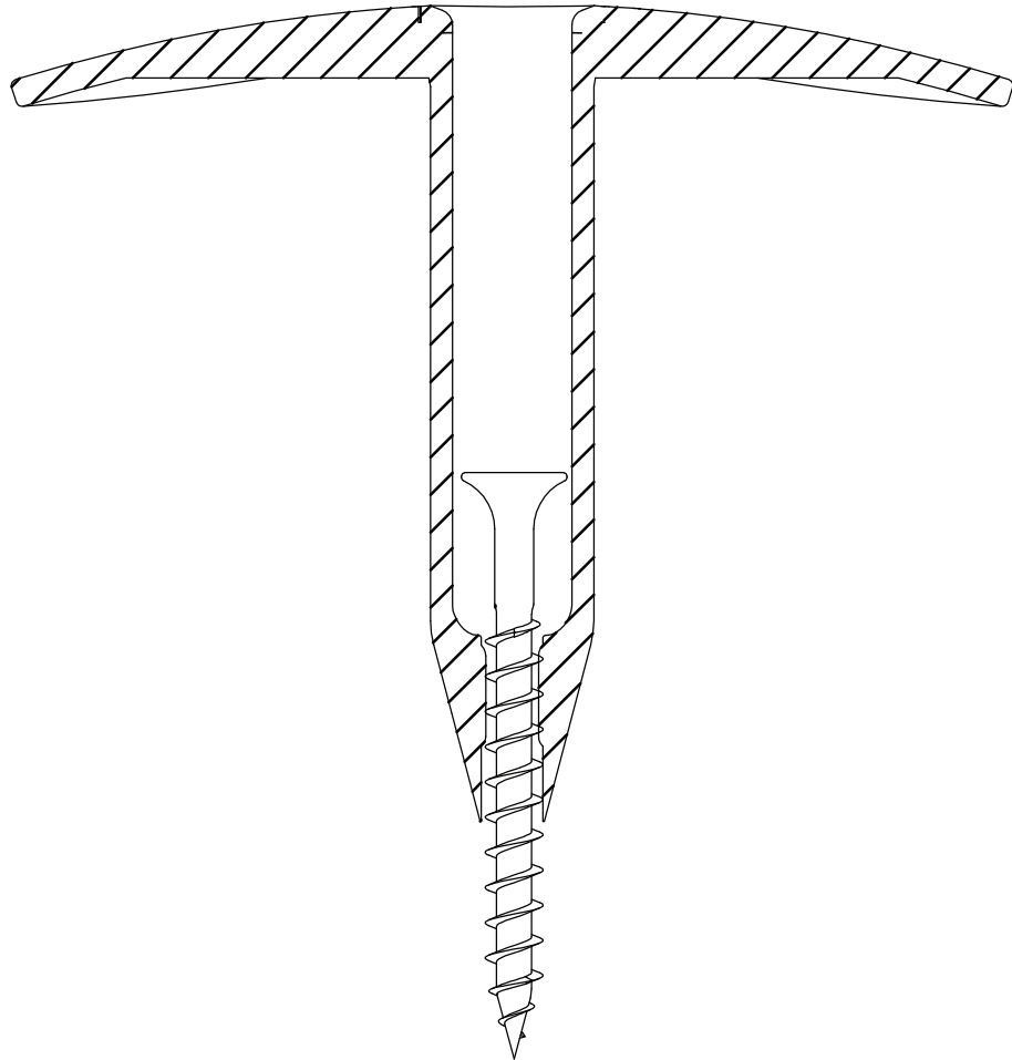
Eurofast EDS-H 5,0 x L
